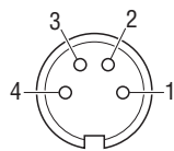
Front side male connector
